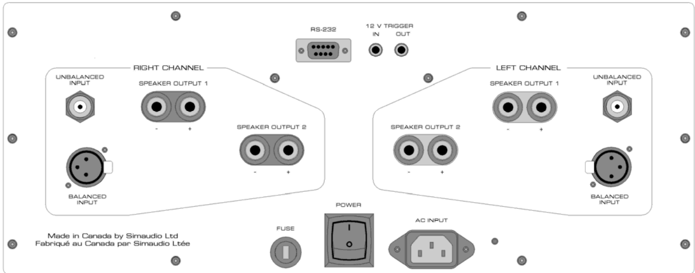
Figure 1: Rear panel of Moon W-8 Dual-Mono Amplifier
