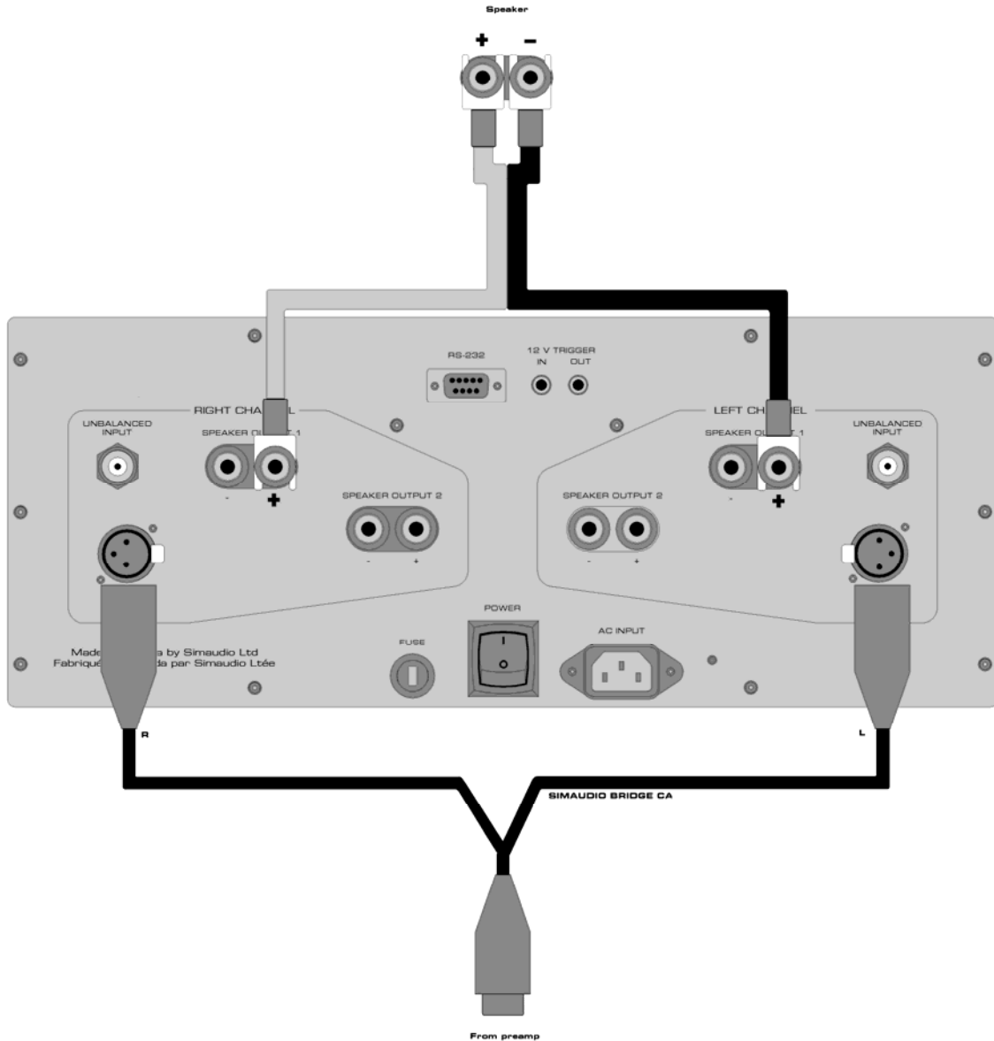
Figure 3: Bridged-Mono operation of the MOON W-8 Dual-Mono Amplifier
