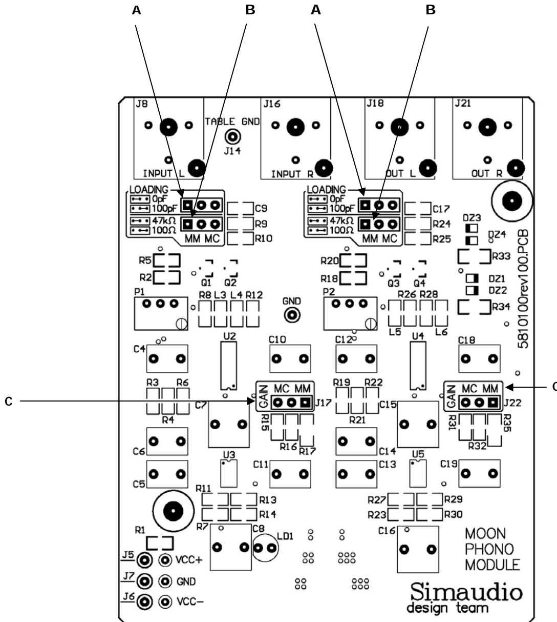
Figure 1: MOON 110LP Circuit Board layout
