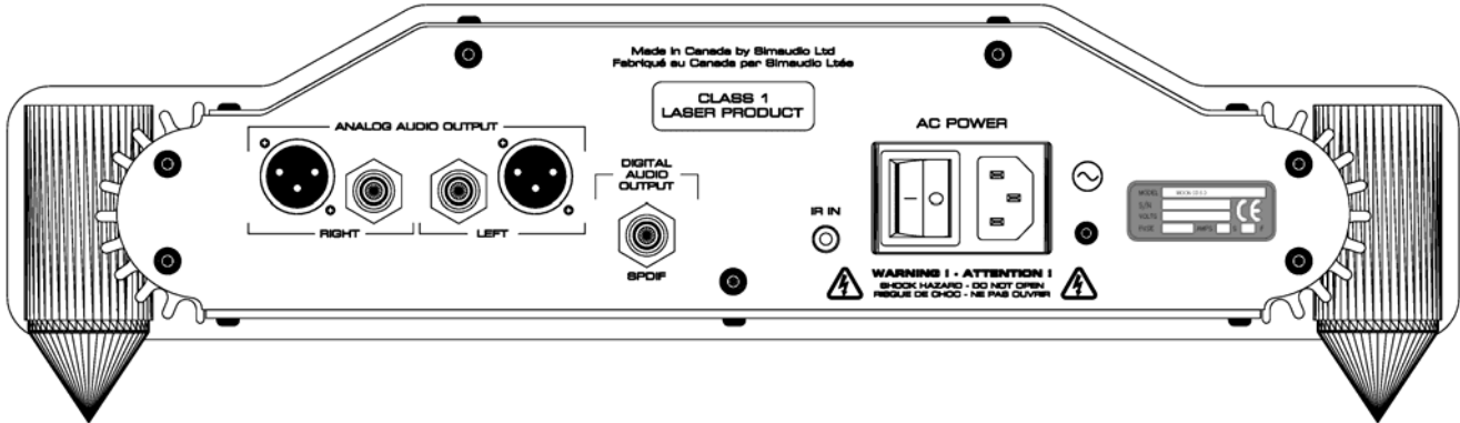
Figure 2: MOON CD 5.3 Rear panel with optional balanced analog outputs
