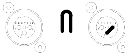
Figure 2: XLR connector without and with jumper accessory
