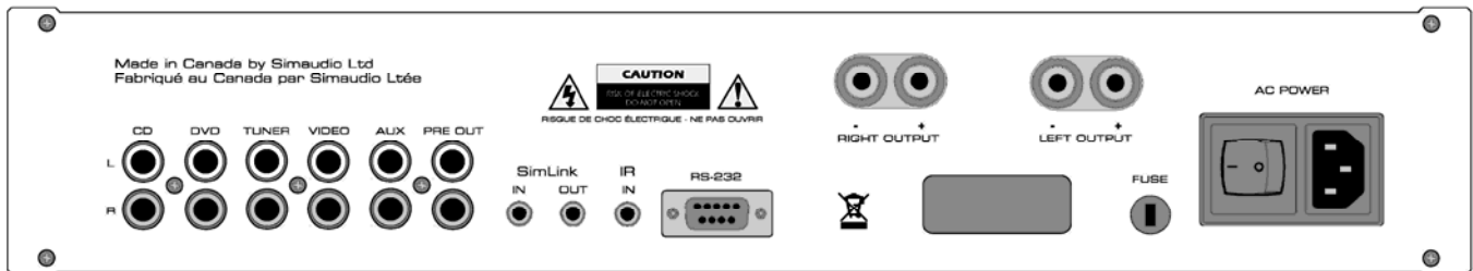
Figure 2: MOON i-1 Rear panel
